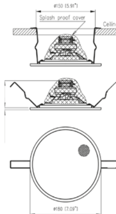
PC-1860EN / PC-1860EN-FTQ
