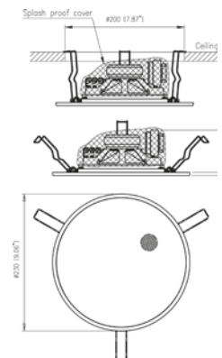
PC-2360EN / PC-2360EN-FTQ
