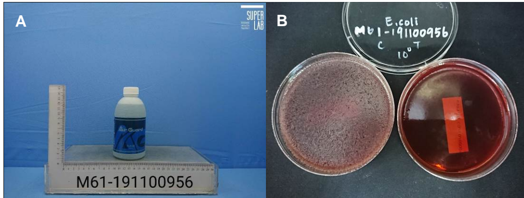
Figure 1. Result of test article (M61-191100956) against Escherichia coli for 30 minutes.
