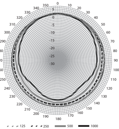
Frequency response
